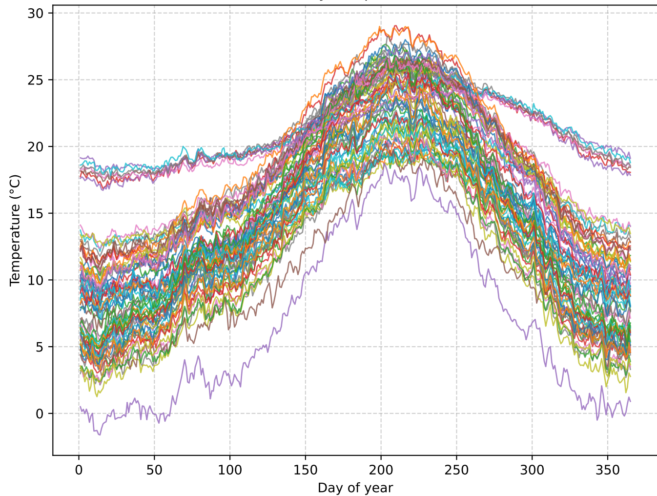
AEMET daily temperature curves
